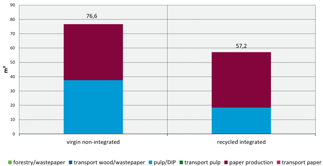
Figure 26: Freshwater Demand, 1000 kg tissue paper, base scenarios
