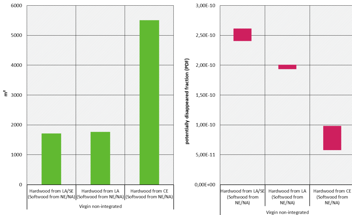
Figure 39: Total forest area (left) and potentially disappeared fraction results shown as range for “low”- and “high”-PDF scenario variants (right), 1000 kg tissue paper (LA = Latin America, SE = Southern Europe, NE = Northern Europe, NA = North America, CE = Central Europe)
