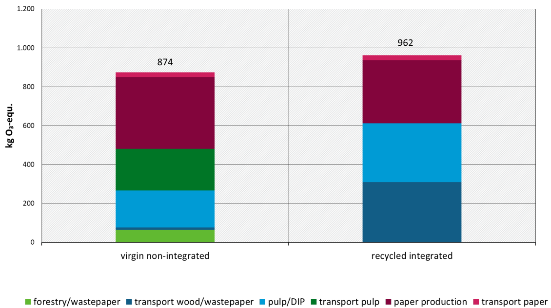
Figure 28: Photochemical Ozone Formation, 1000 kg tissue paper, base scenarios
