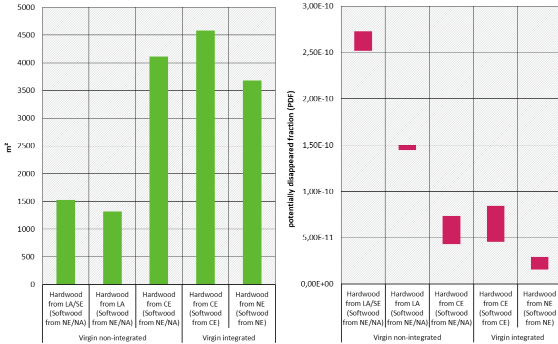
Figure 38: Total forest area (left) and potentially disappeared fraction results shown as range for “low”- and “high”-PDF scenario variants (right), 1000 kg office paper (LA = Latin America, SE = Southern Europe, NE = Northern Europe, NA = North America, CE = Central Europe)
